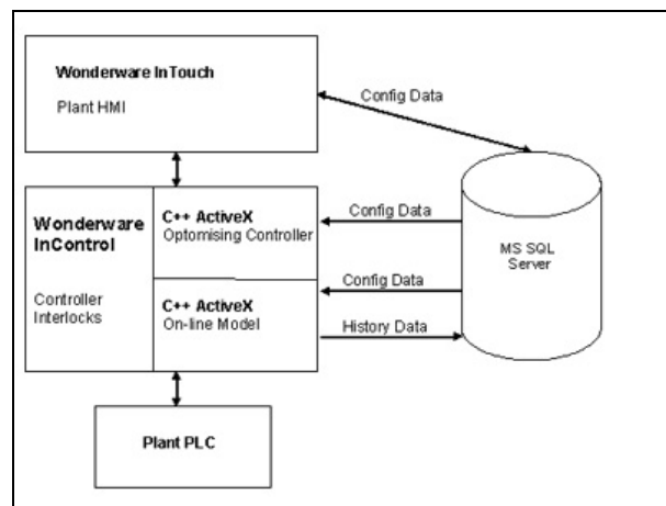
Figure 4 – Layout of implemented advanced process control system.
