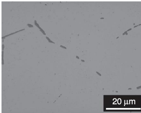
Figure 2 - Example microstructure after homogenising 3 .
