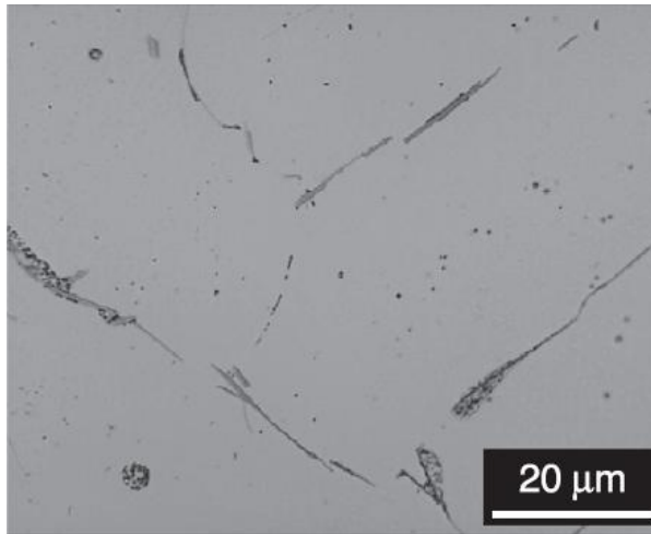
Figure 1 - Example microstructure before homogenising 3 .
