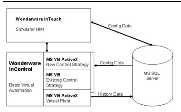
Figure 3 – Simulator system layout.
