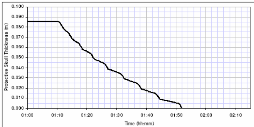
Figure 11: Skull thickness for scenario 2
