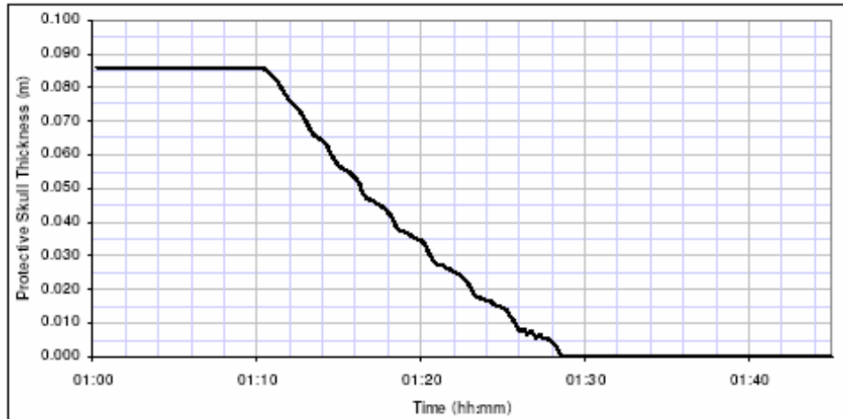
Figure 10: Skull thickness for scenario 1
