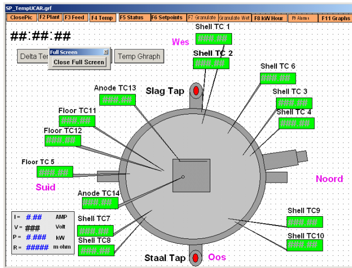
Figure 9: Thermocouple arrangement on a pilot scale furnace
