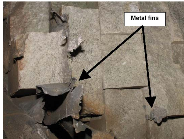
Figure 2: Iron penetration into the hearth found after a refractory break-out on a DC-ilmenite smelter [3]
