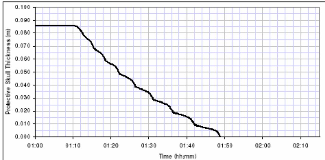
Figure 12: Skull thickness for scenario 3
