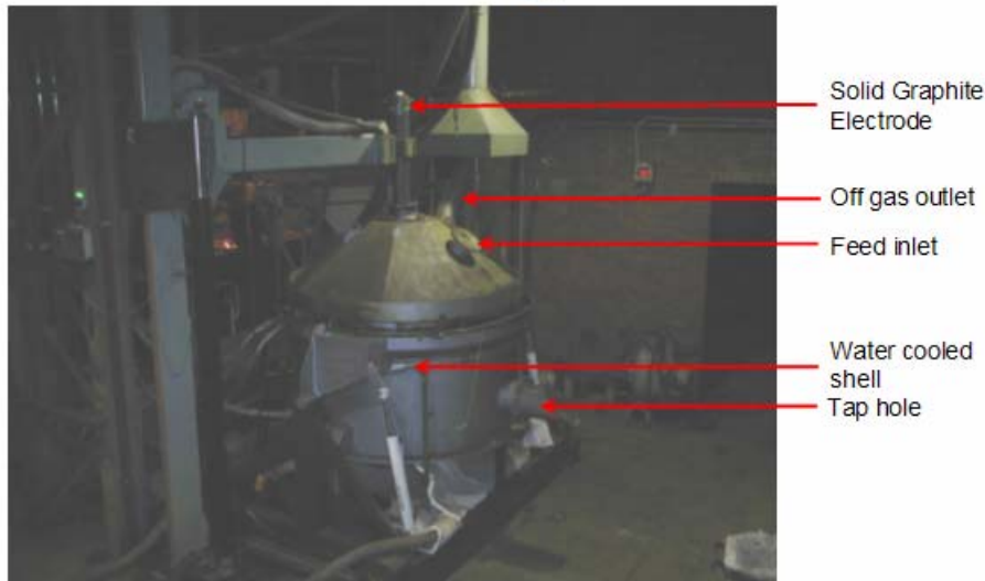
Figure 6: A photo of the 500 kW furnace set-up
