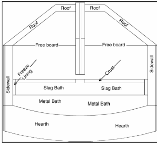
Figure 4: Schematic of the furnace and process as described by the Furnace Model [5]
