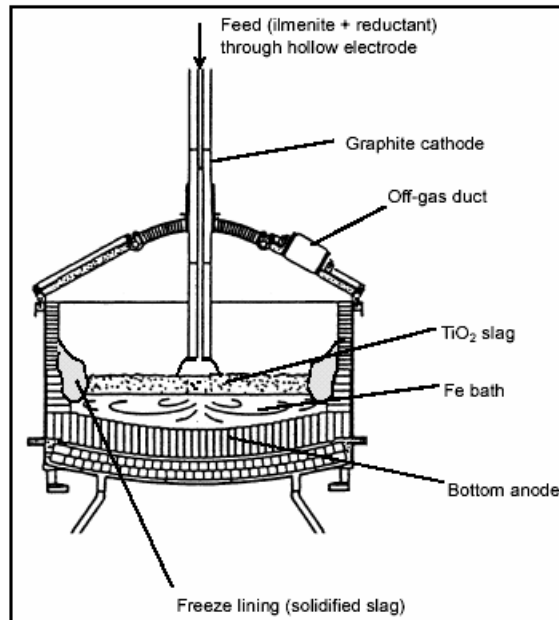
Figure 1: Typical Ilmenite-smelting furnace [4]
