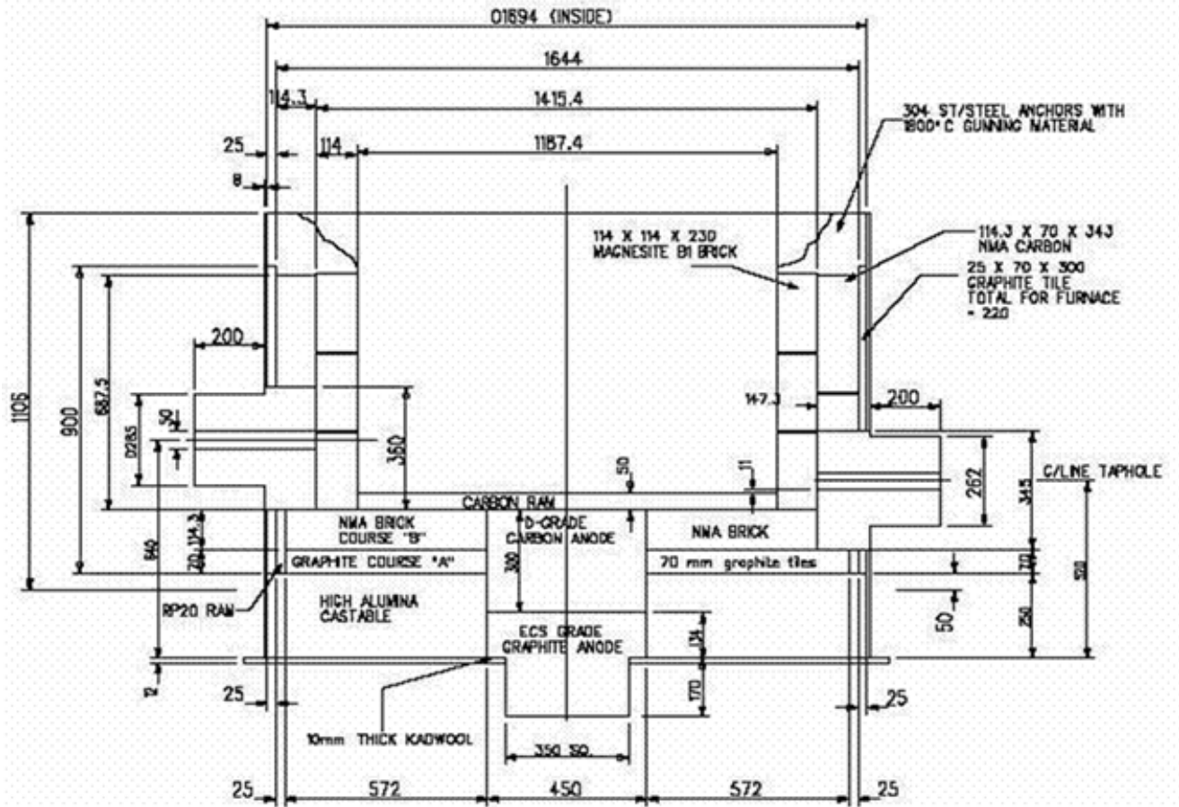
Figure 5: Drawing of the 500kW pilot scale furnace showing the UCAR® CHILL-KOTE™ Lining
