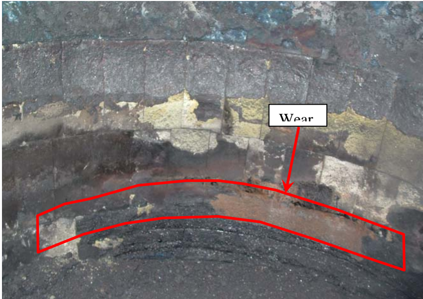
Figure 7: View of the refractory lining after the furnace was cleaned out.
